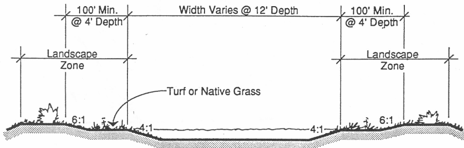
FIGURE 6-4 DETENTION POND SECTION
